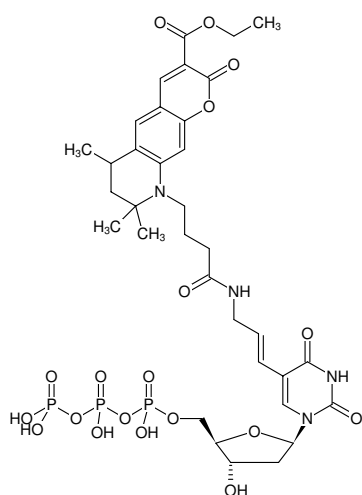
Structural formula of Atto425 NT Labeling Kit
