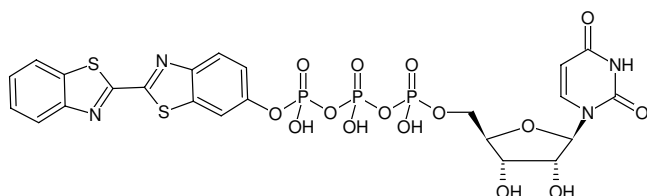
Structural formula of γ-(BBT)-UTP
