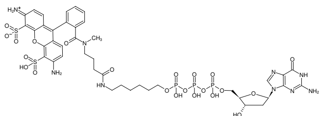
Structural formula of \gamma -(6-Aminoethyl)-dGTP-ATTO-488
