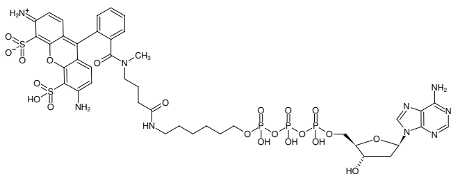
Structural formula of \gamma -(6-Aminoethyl)-dATP-ATTO-488
