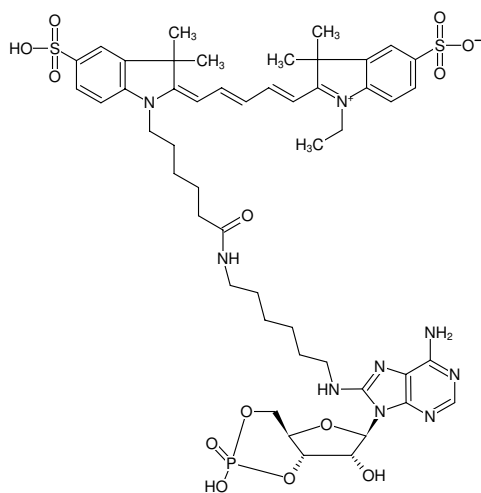
Structural formula of 8-(6-Aminoethyl)-amino-cAMP-Cy5
