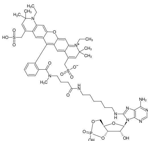
Structural formula of 8-(6-Aminoethyl)-amino-cAMP-ATTO-594
