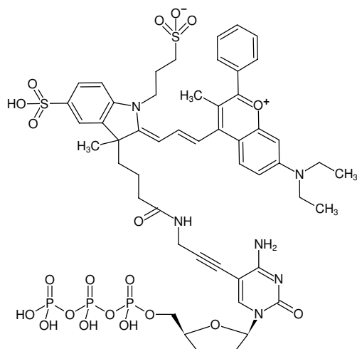
Structural formula of 5-Propargylamino-ddCTP-DYQ-661
