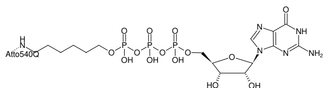
Structural formula of \gamma -(6-Aminoethyl)-GTP-ATTO-540Q
