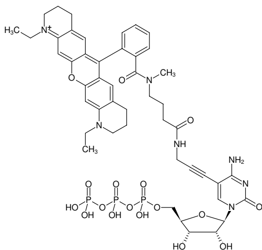
Structural formula of 5-Propargylamino-CTP-ATTO-Rho11
