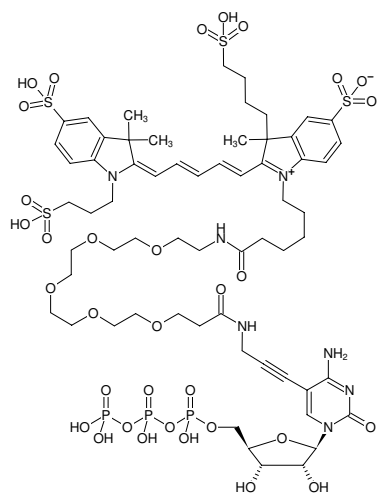
Structural formula of 5-Propargylamino-CTP-PEG 5 -AF647
