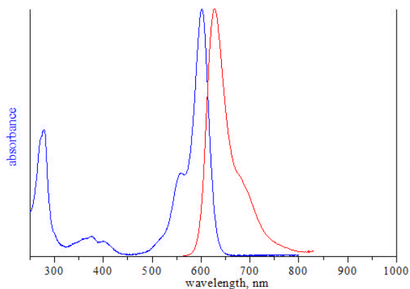
excitation and emission spectrum of AF594
