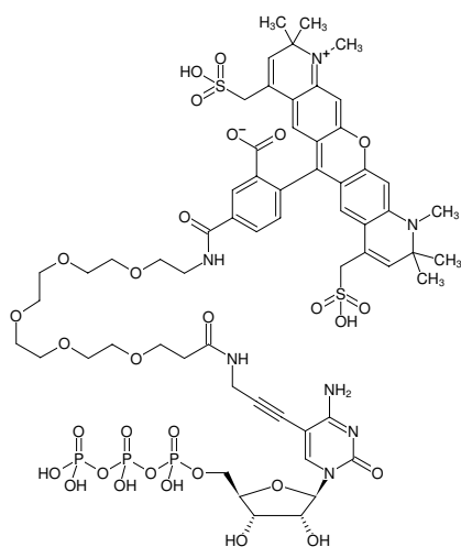
Structural formula of 5-Propargylamino-CTP-PEG 5 -AF594
