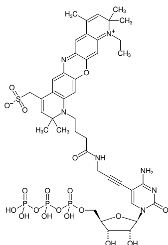
Structural formula of 5-Propargylamino-CTP-ATTO-700
