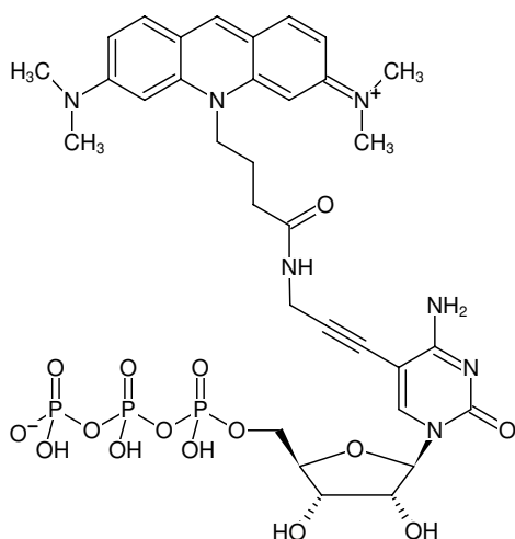
Structural formula of 5-Propargylamino-CTP-ATTO-495
