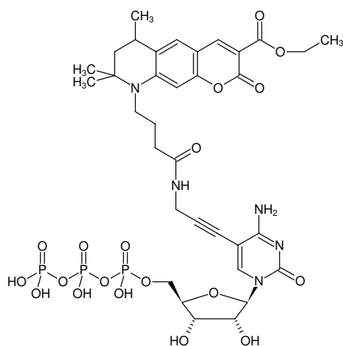
Structural formula of 5-Propargylamino-CTP-ATTO-425
