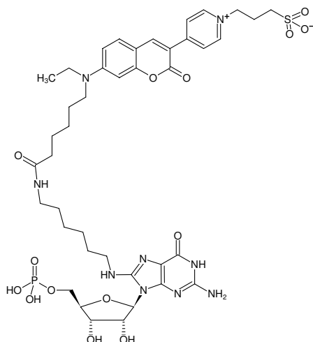
Structural formula of 8-(6-Aminoethyl)-amino-GMP-DY-485XL
