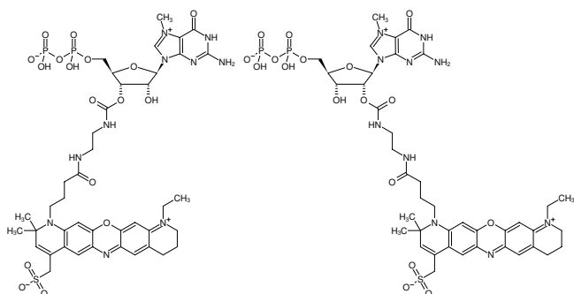
Structural formula of EDA-m 7 GDP-ATTO-680
