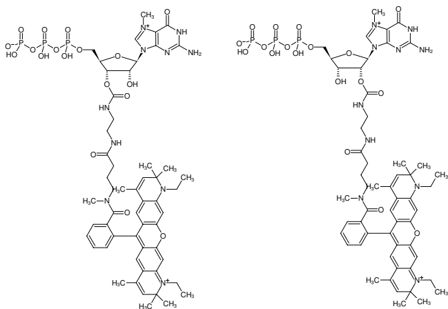
Structural formula of EDA-m 7 GTP-ATTO-Rho13
