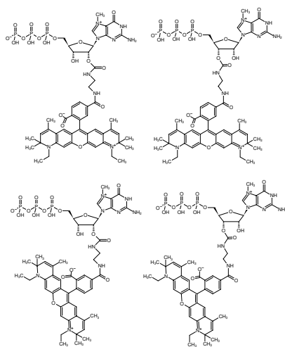
Structural formula of EDA-m 7 GTP-ATTO-590
