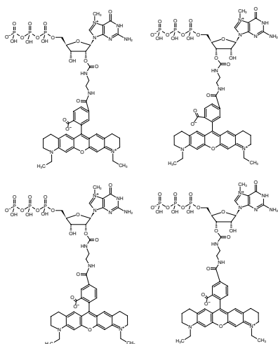
Structural formula of EDA-m 7 GTP-ATTO-565
