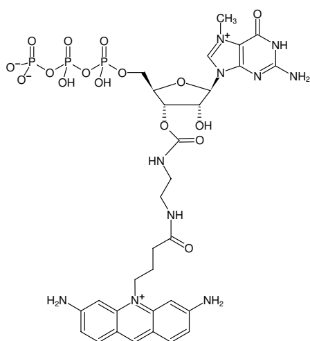
Structural formula of EDA-m 7 GTP-ATTO-465
