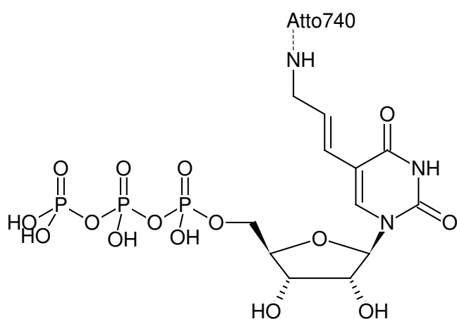
Structural formula of Aminoallyl-UTP-ATTO-740
