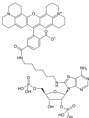
Structural formula of 8-(6-Aminoethyl)-amino-adenosine-2',5'-bisphosphate-6-ROX
