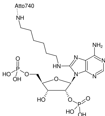
Structural formula of 8-(6-Aminoethyl)-amino-adenosine-2',5'-bisphosphate-ATTO-740
