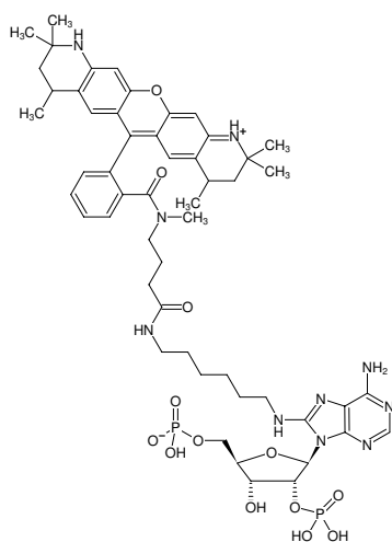
Structural formula of 8-(6-Aminoethyl)-amino-adenosine-2',5'-bisphosphate-ATTO-550
