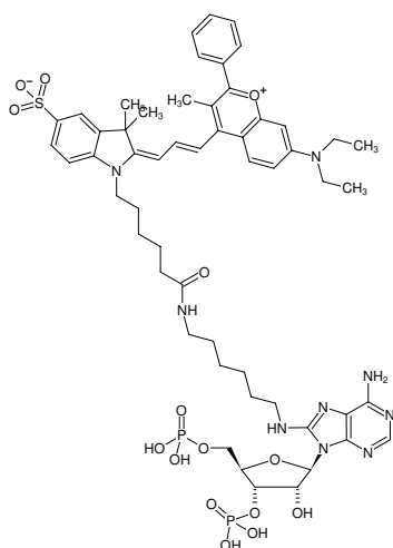
Structural formula of 8-(6-Aminoethyl)-amino-adenosine-3',5'-bisphosphate-DYQ-660
