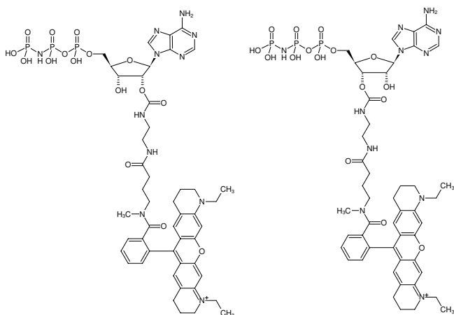
Structural formula of EDA-AppNHp (EDA-AMPPNP)-ATTO-Rho11
