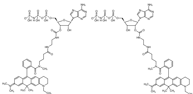
Structural formula of EDA-AppNHp (EDA-AMPPNP)-ATTO-633
