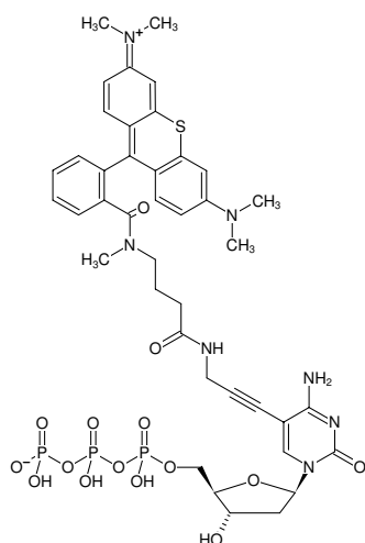
Structural formula of 5-Propargylamino-dCTP-ATTO-Thio12
