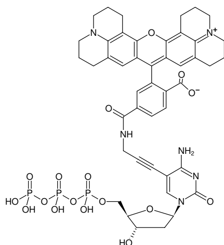
Structural formula of 5-Propargylamino-dCTP-6-ROX
