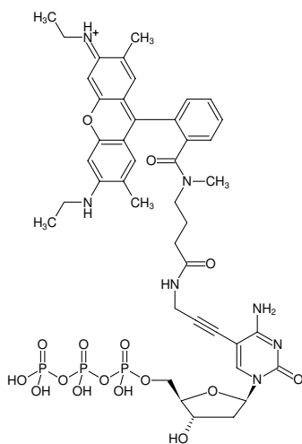
Structural formula of 5-Propargylamino-dCTP-ATTO-Rho6G
