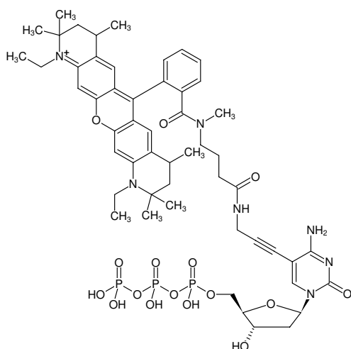
Structural formula of 5-Propargylamino-dCTP-ATTO-Rho12
