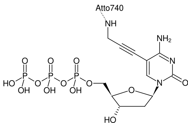
Structural formula of 5-Propargylamino-dCTP-ATTO-740
