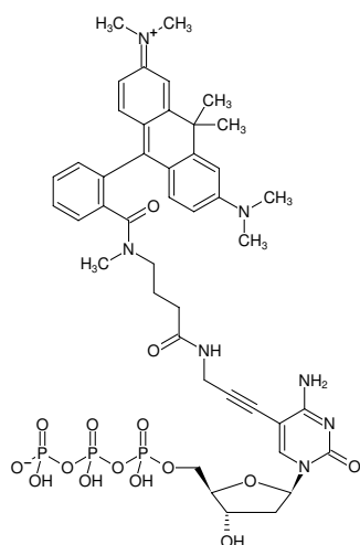
Structural formula of 5-Propargylamino-dCTP-ATTO-620
