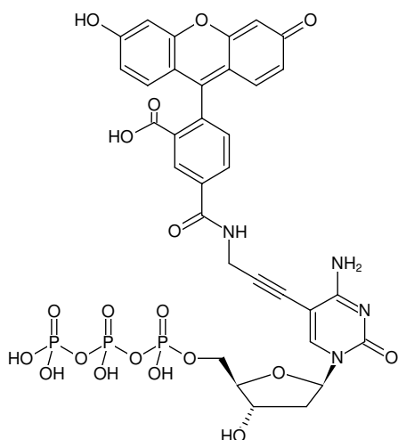
Structural formula of 5-Propargylamino-dCTP-5-FAM
