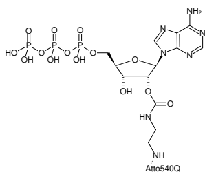
Structural formula of EDA-ATP-ATTO-540Q
