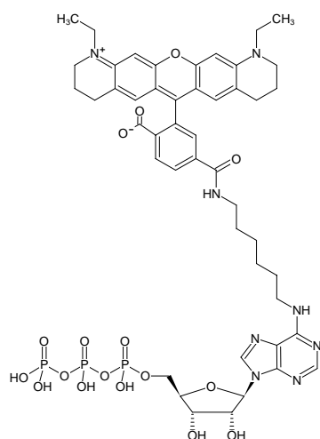
Structural formula of N 6 -(6-Aminoethyl)-ATP-ATTO-565
