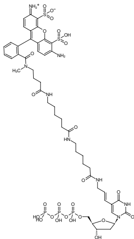
Structural formula of Aminoallyl-dUTP-XX-ATTO-488
