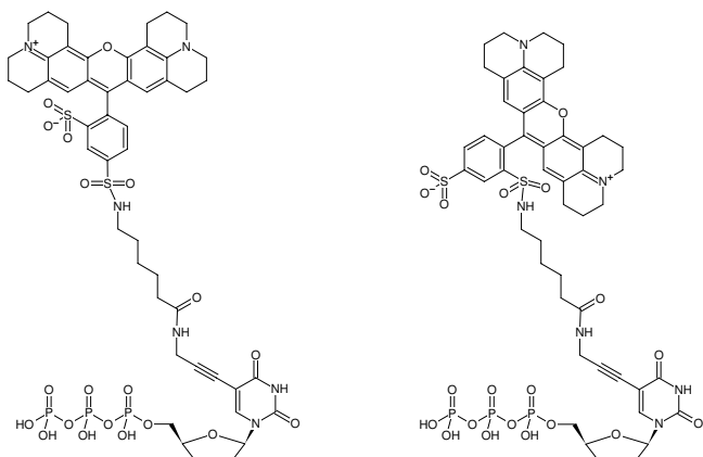
Structural formula of 5-Propargylamino-ddUTP-Texas Red
