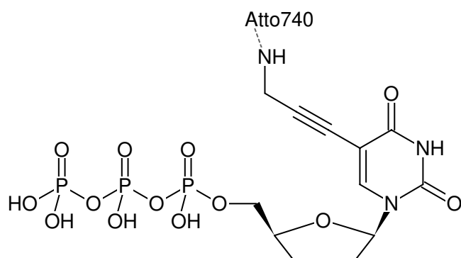
Structural formula of 5-Propargylamino-ddUTP-ATTO-740
