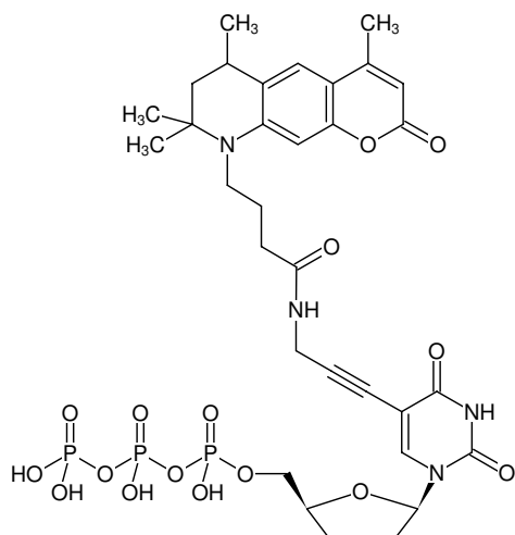
Structural formula of 5-Propargylamino-ddUTP-ATTO-390
