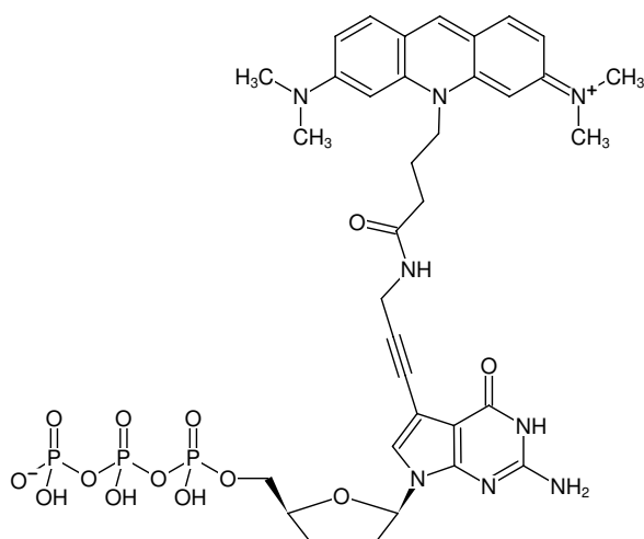
Structural formula of 7-Propargylamino-7-deaza-ddGTP-ATTO-495
