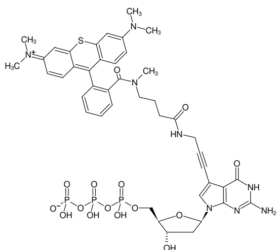
Structural formula of 7-Propargylamino-7-deaza-dGTP-ATTO-Thio12
