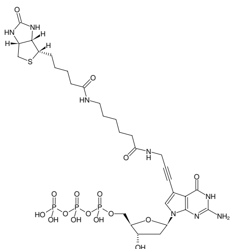
Structural formula of Biotin-11-dGTP
