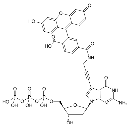
Structural formula of 7-Propargylamino-7-deaza-dGTP-6-FAM
