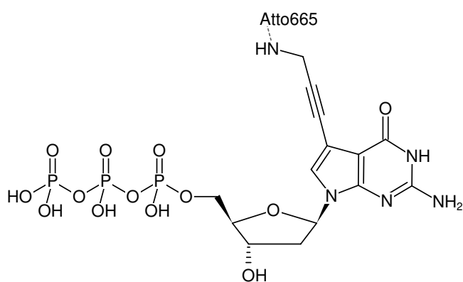
Structural formula of 7-Propargylamino-7-deaza-dGTP-ATTO-665
