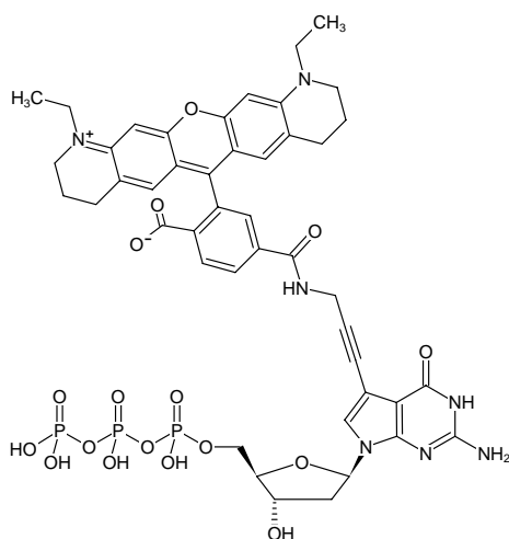
Structural formula of 7-Propargylamino-7-deaza-dGTP-ATTO-565
