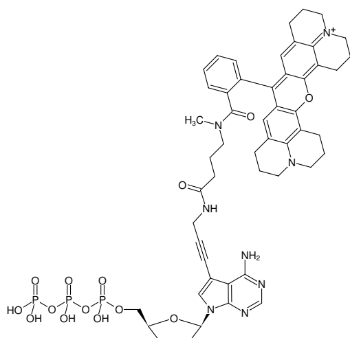
Structural formula of 7-Propargylamino-7-deaza-ddATP-ATTO-Rho101
