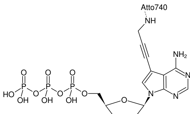
Structural formula of 7-Propargylamino-7-deaza-ddATP-ATTO-740
