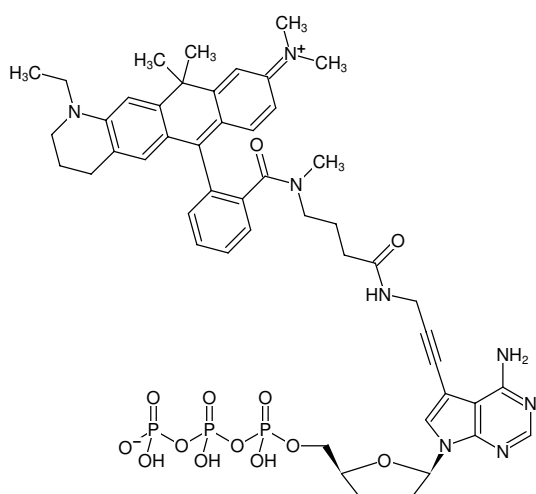
Structural formula of 7-Propargylamino-7-deaza-ddATP-ATTO-633
