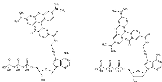
Structural formula of 7-Propargylamino-7-deaza-dATP-5/6-TAMRA
